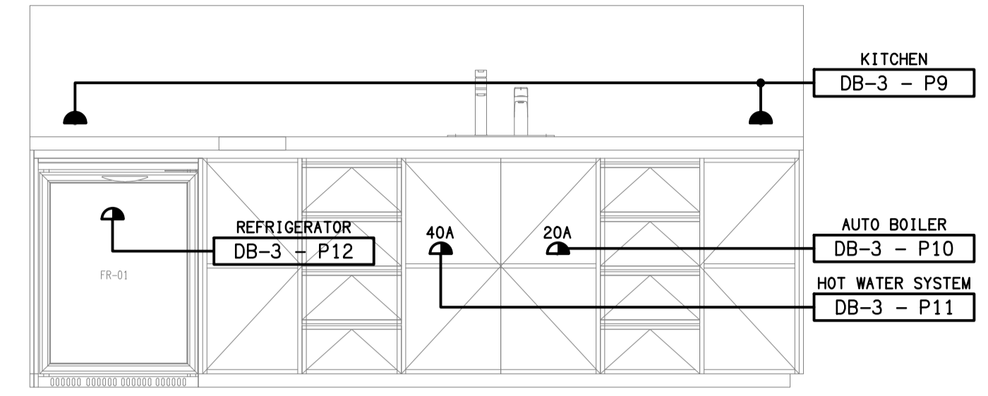
DETAIL A CUSTOMER KITCHENETTE ELEVATION SCALE 1: 20
